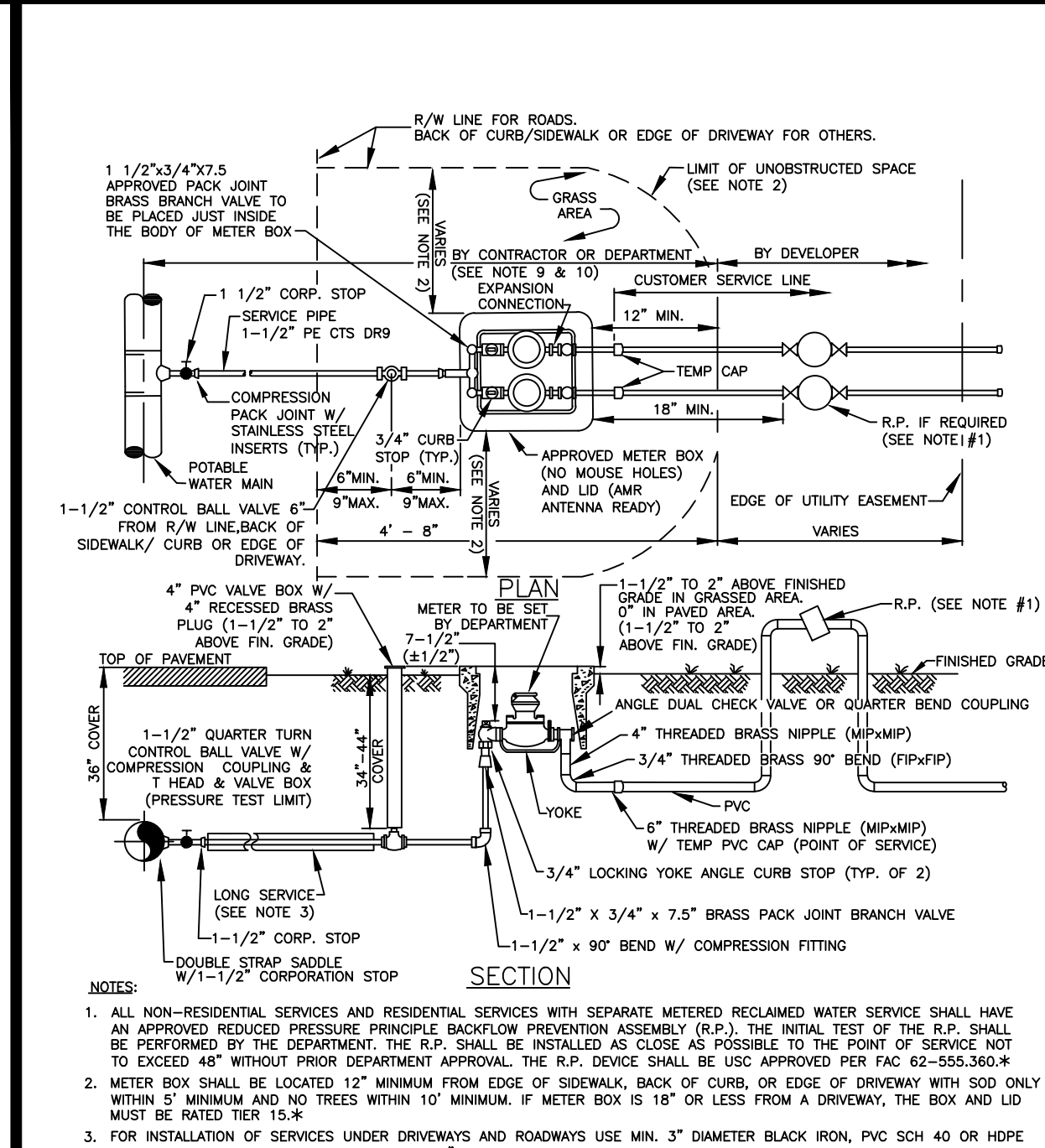
POTABLE WATER SERVICE DUAL 5/8\"/>
