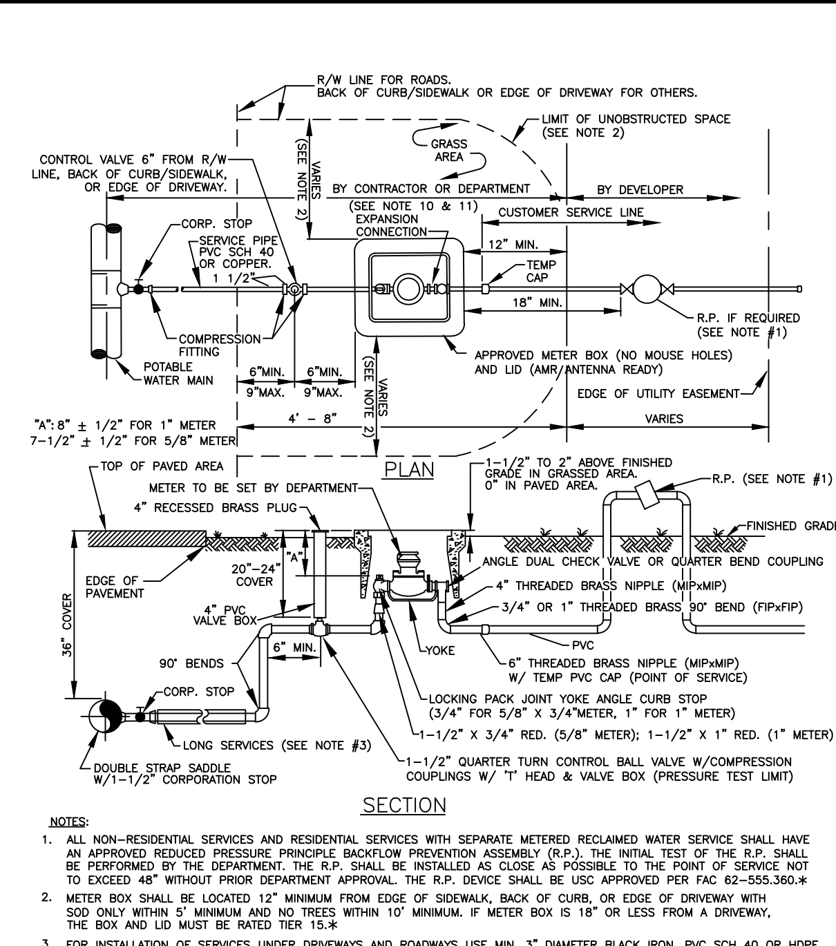
POTABLE WATER SERVICE SINGLE 5/8\"/>
