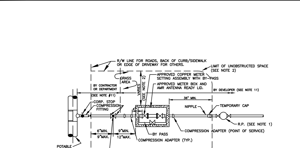
POTABLE WATER 3\"/>
