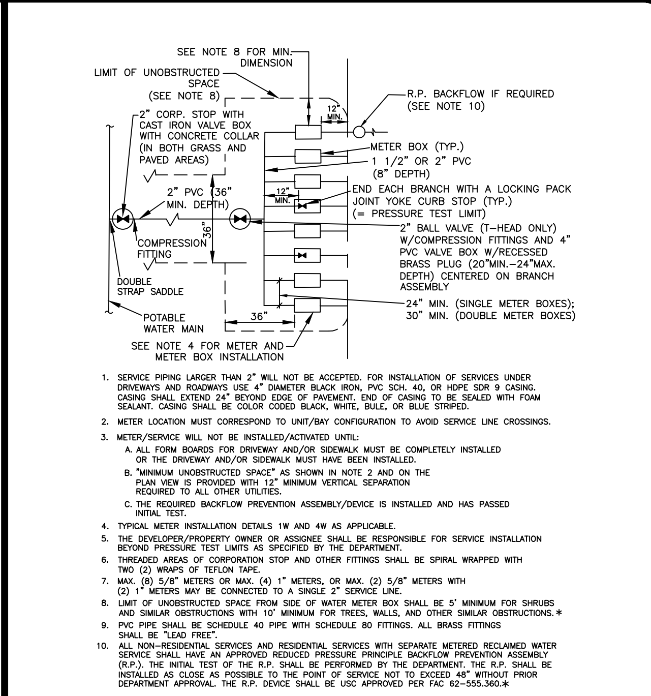
POTABLE WATER TYPICAL CONNECTION FOR MULTIPLE SERVICES * 5W
