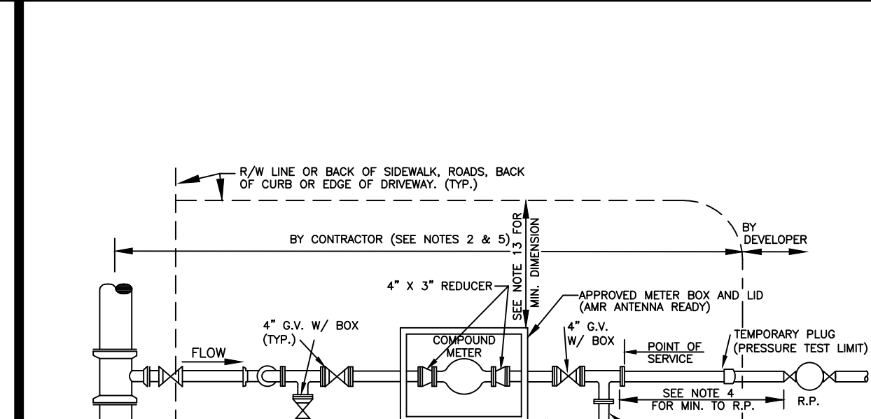
POTABLE WATER 3\"/>
