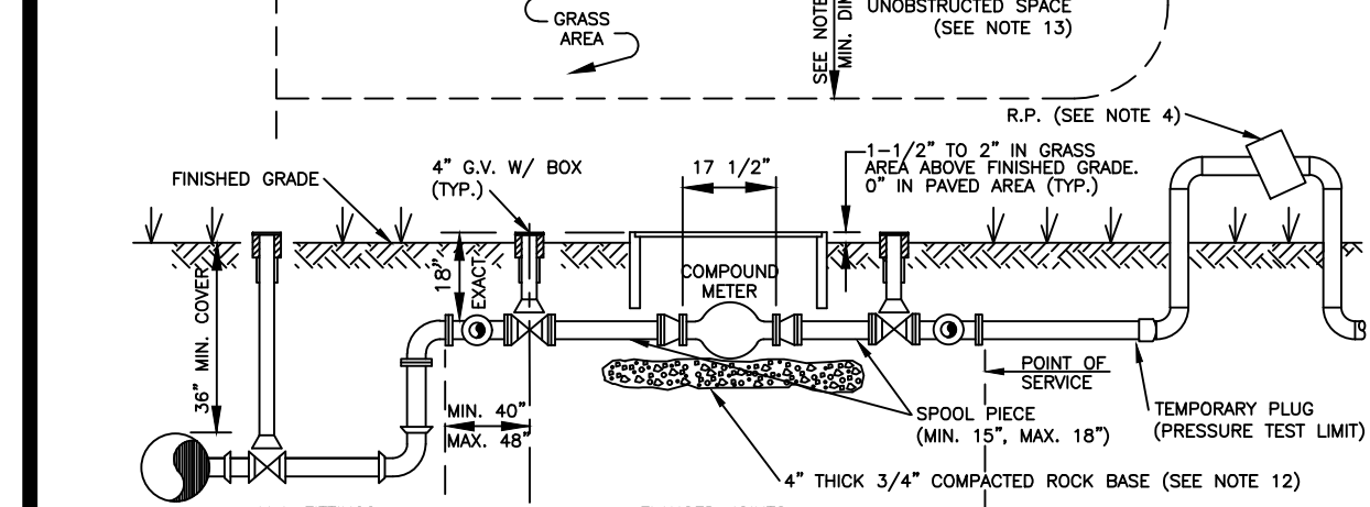
POTABLE WATER 3\"/>
