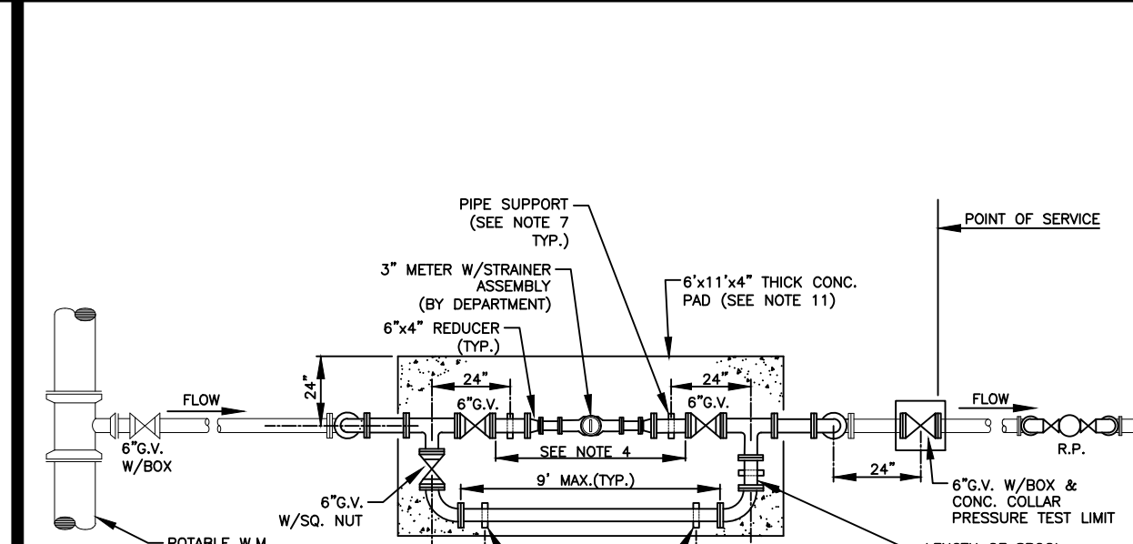
POTABLE WATER 3\"/>
