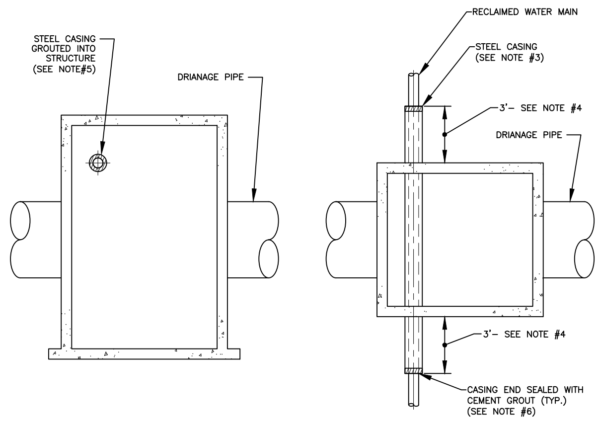
PROFILE PLAN
