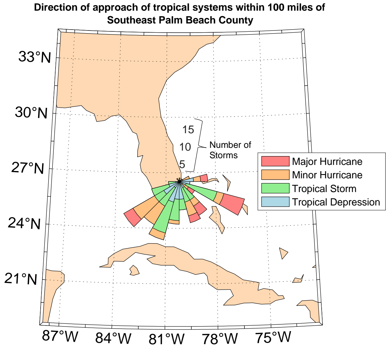
Figure 1-13. Historic direction of approach of tropical systems (Data Source: NOAA 2016).
