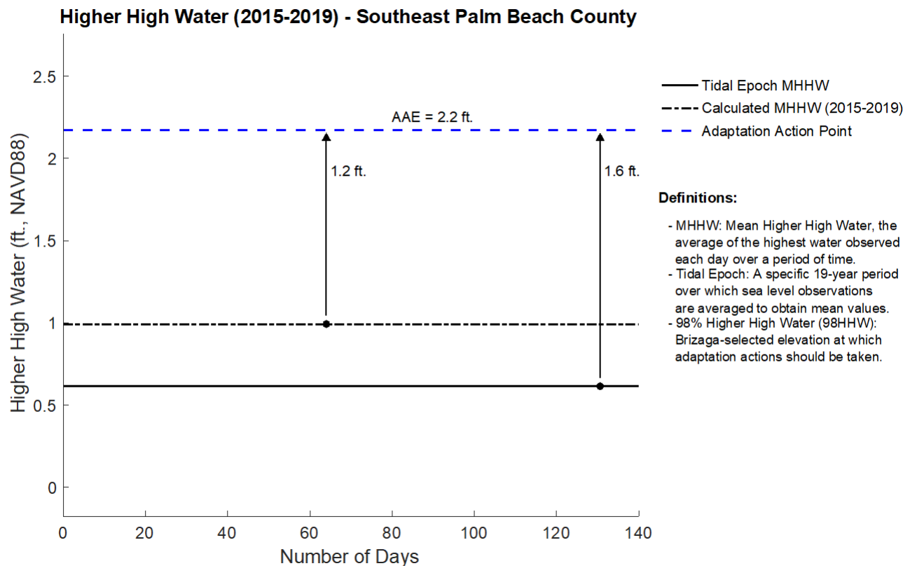
Figure 1-31. Histogram of Higher High Water, with the calculated Adaptation Action Elevation for the year 2020.
