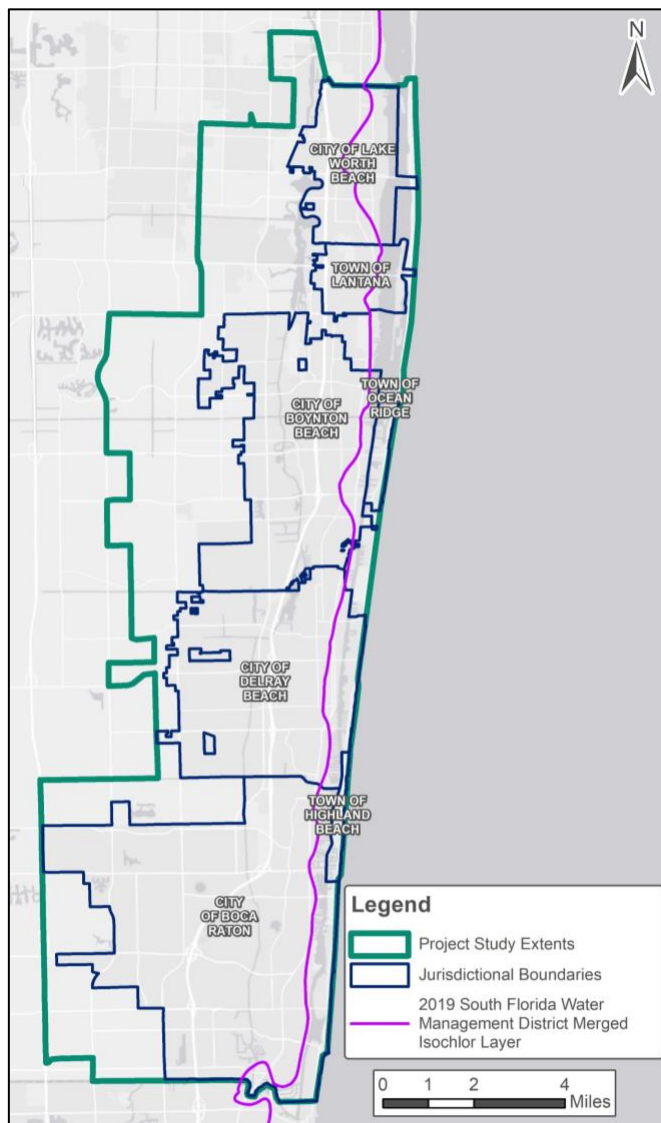
Figure 2-13. South Florida Water Management District's 2019 Isochlor (Data Source: SFWMD, 2020).
