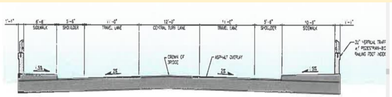
Proposed Typical Bridge Cross Section
