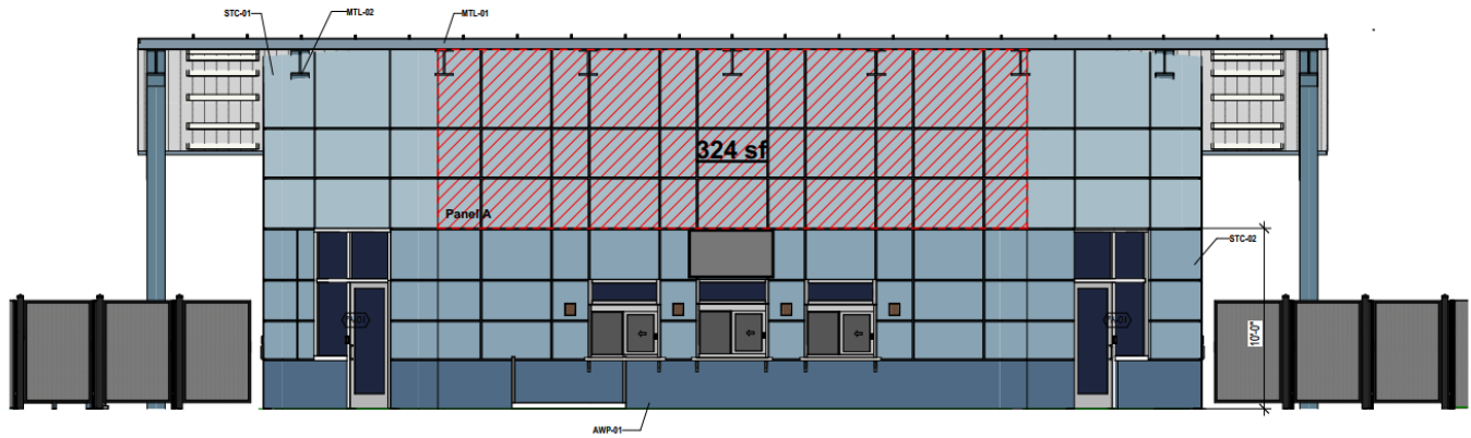
① EXTERIOR ELEVATION - SOUTH AWP 1/4" = 1'-0"
