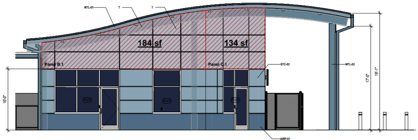
② EXTERIOR ELEVATION - WEST 1/4" = 1'-0"
