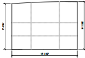
⑥ AWP - PANEL C.1/C.2, 134 SF 1/4" = 1'-0" (STUCCO APPLIED TO TILE-UP CONCRETE PANEL)
