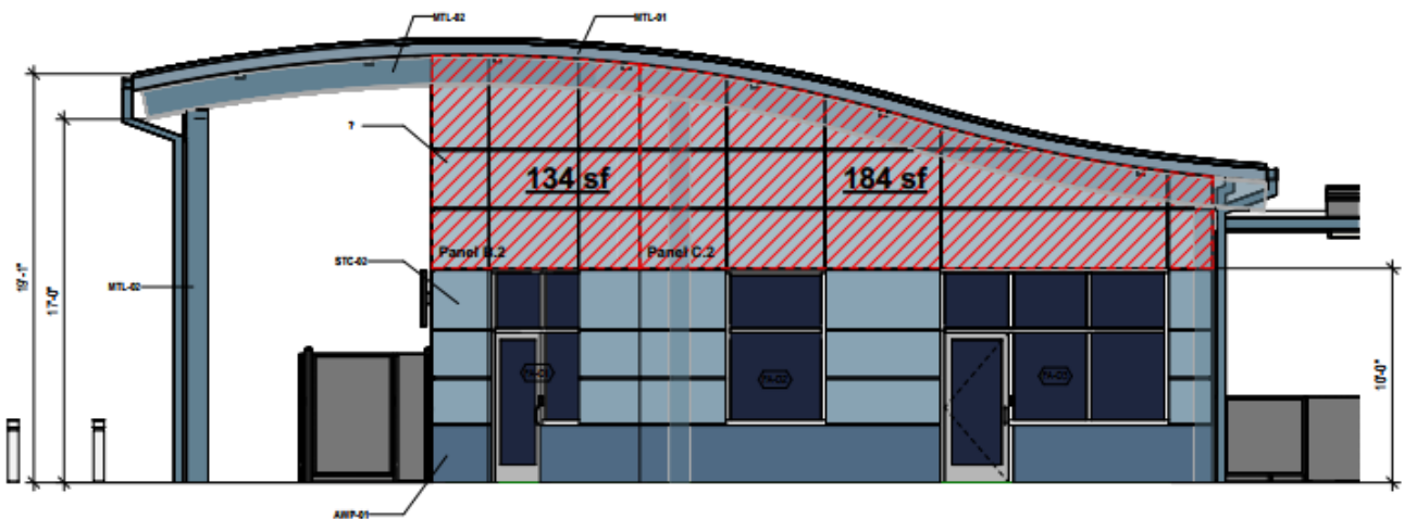
③ EXTERIOR ELEVATION - EAST 1/4" = 1'-0"
