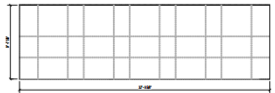
⑦ AWP - PANEL A, 324 1/4" = 1'-0" (STUCCO APPLIED TO TILE-UP CONCRETE PANEL)
